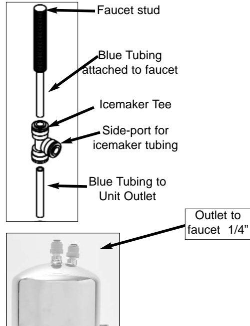
Connecting icemaker to stainless steel unit
